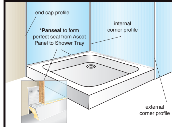
Typical Corner Sited Installation
