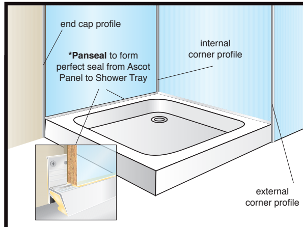
Typical Corner Sited Installation
