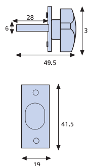
Easi-Turn
